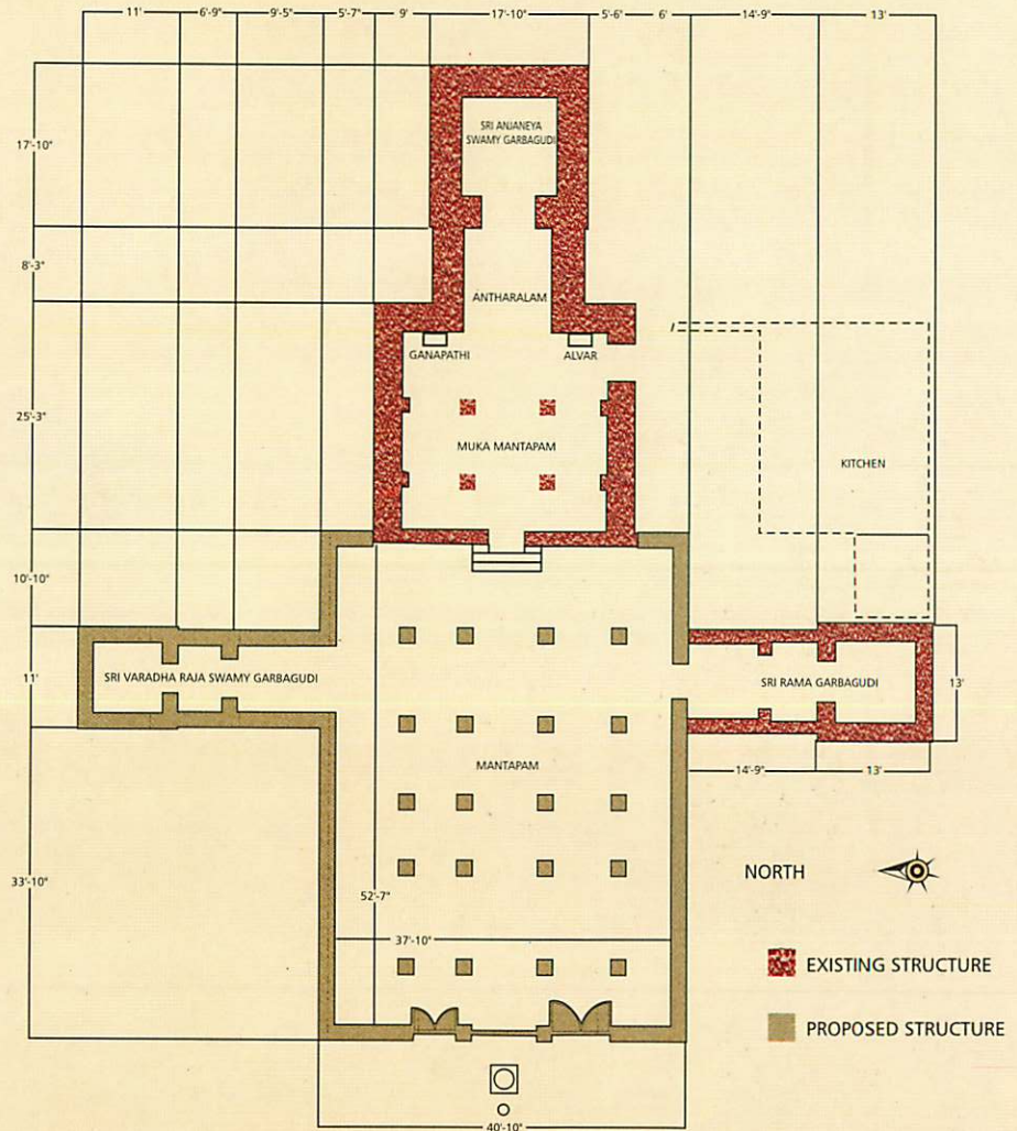
Plan showing the Existing temple of Sri Anjaneya Swamy, Mulbagal
