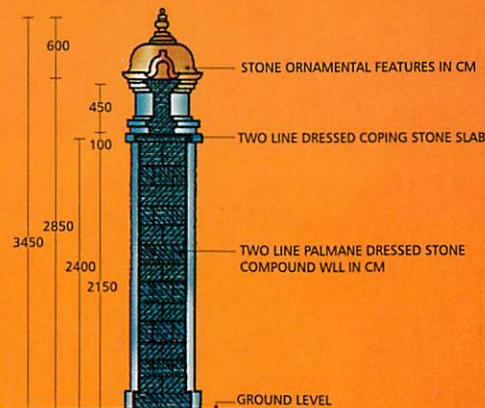
Proposed front Elevation of Vahana Mantapa
